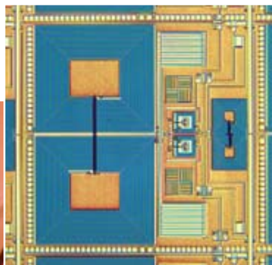
ARRAY OF SENSORS ( below ) will be bonded to a SQUID multiplexer chip. The detail at the left shows one pixel of the multiplexer.
